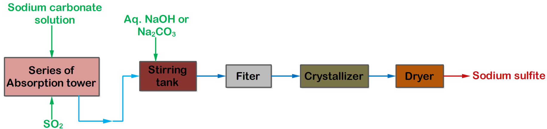
Figure: Manufacture of Sodium sulfite from soda ash and sulfur dioxide
